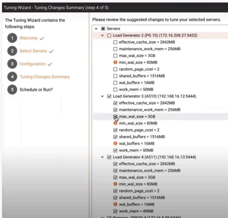
TUNING WIZARD IN POSTGRES ENTERPRISE MANAGER
